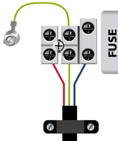
Figure 3: AC Power Wiring
