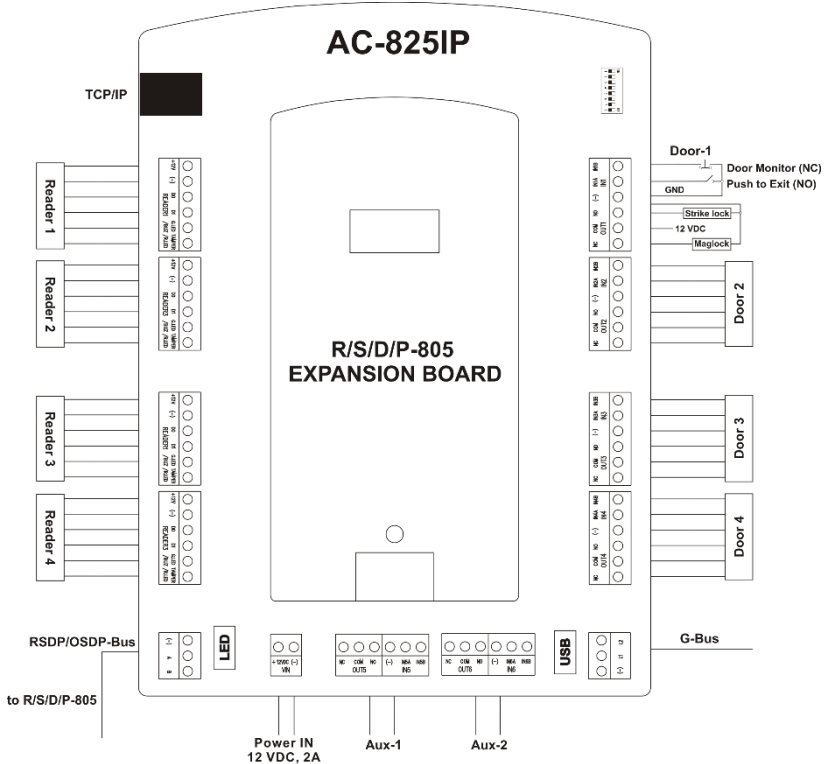
Figure 8: AC-825IP Wiring Communications
