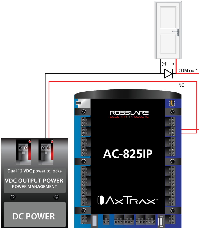
Figure 6: Door Lock – Failed Open
