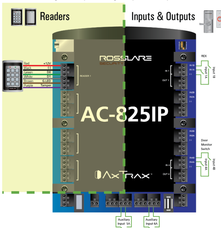
Figure 4: Input Wiring – Supervised Inputs
